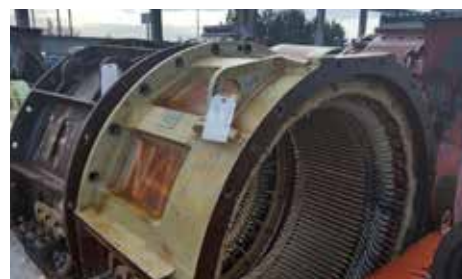
CARCASSE-STATOR - AT 5
